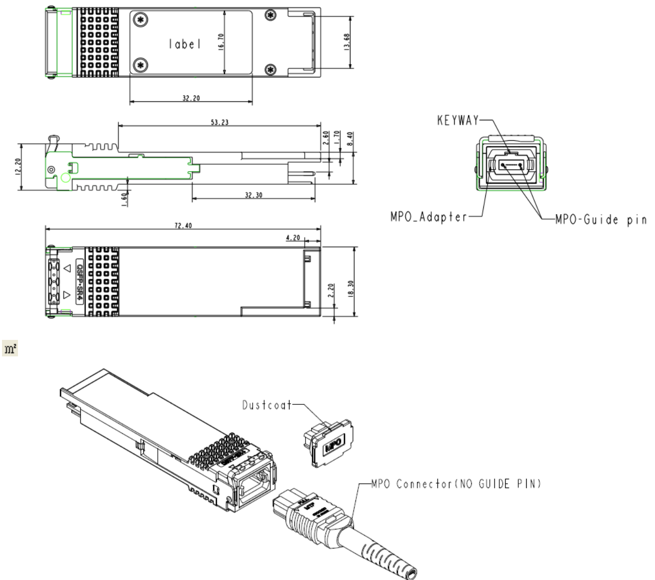
Figure10. Mechanical Specifications
